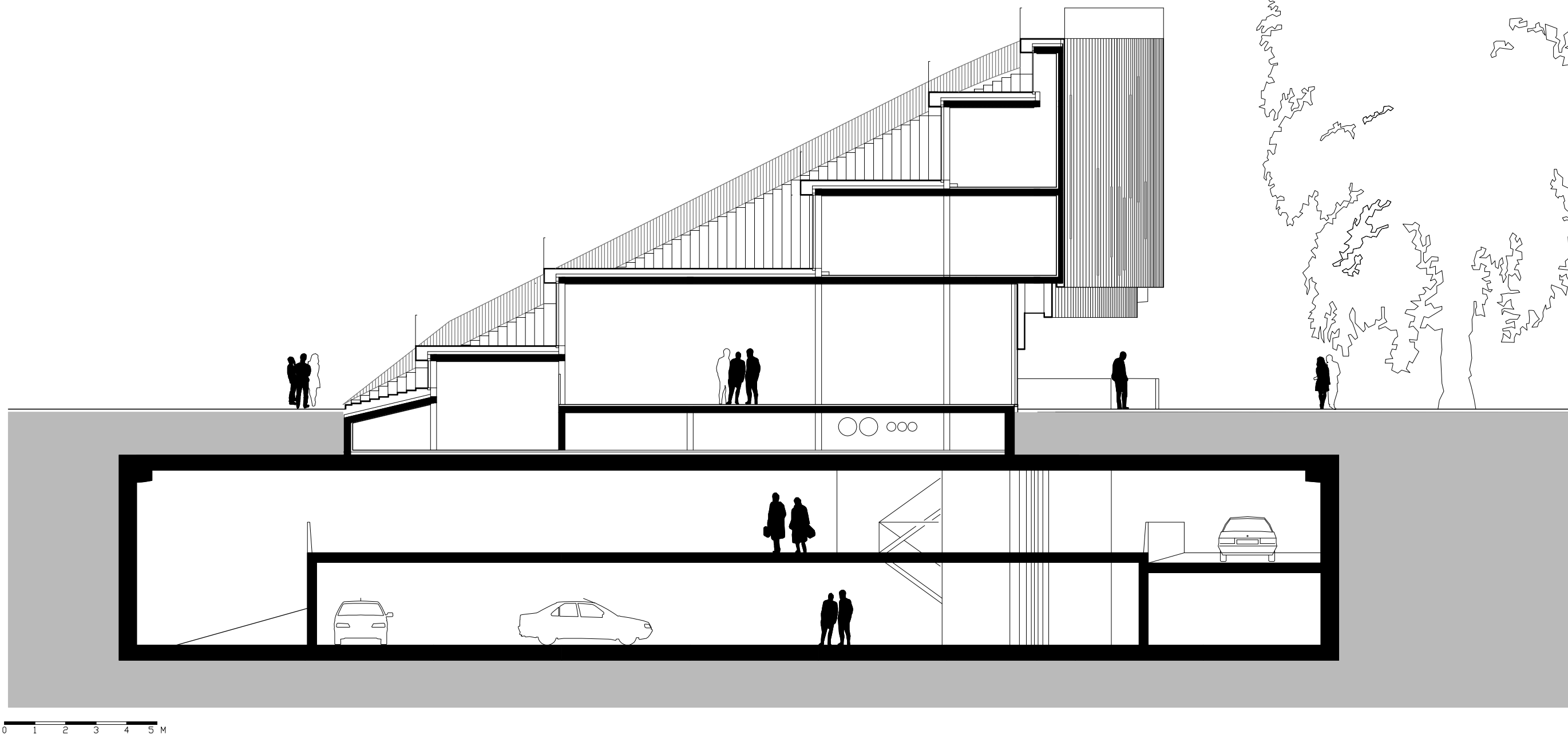
section 1 Pavillion - Roosendaal
