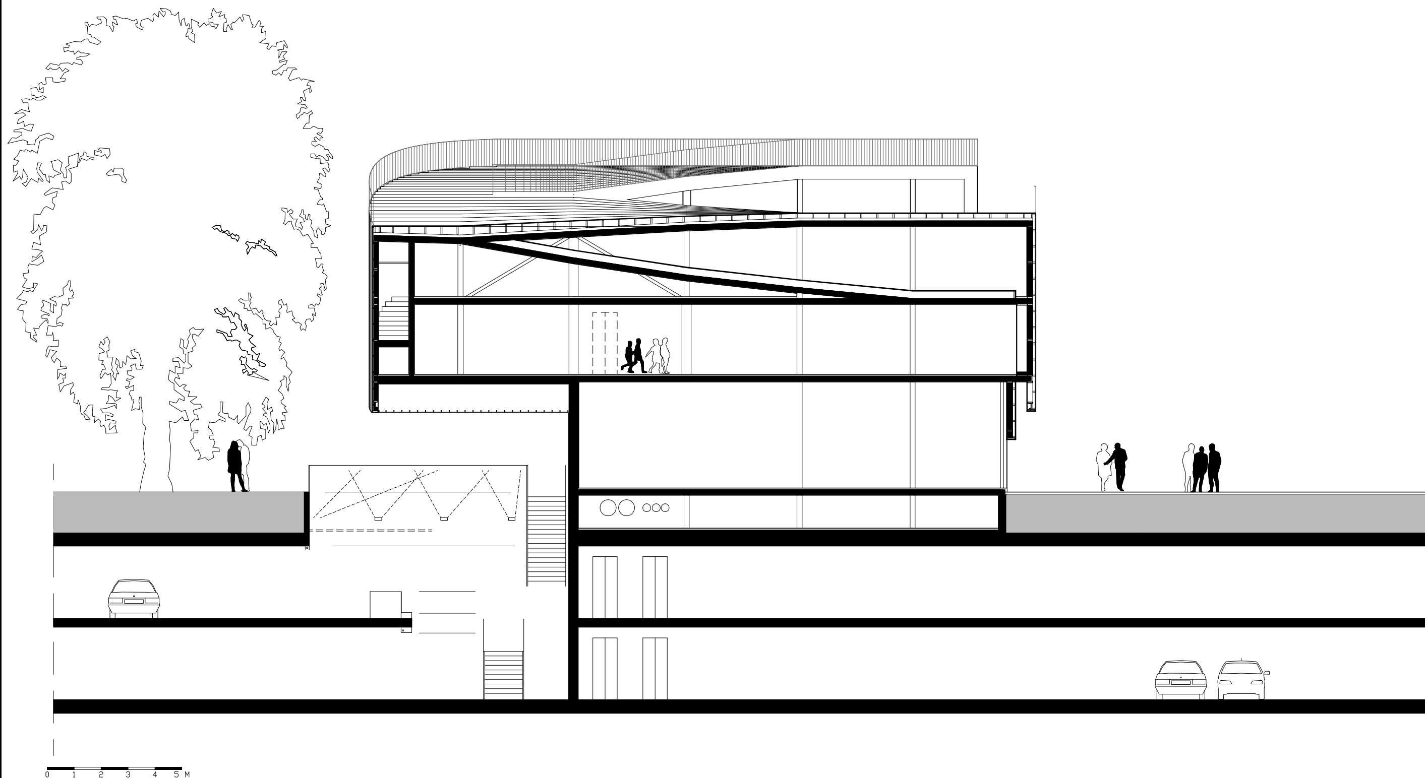
section 5 Pavillion - Roosendaal
